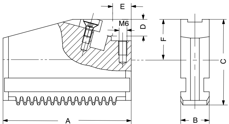
Tool group C 21 Type 545-30 Draw-down jaws, for interchangeable clamping inserts, straight toothing , 1 piece, without clamping inserts
