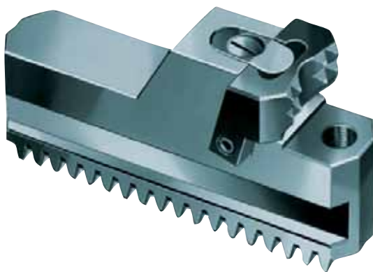
Tool group C 21 Type 545-30 Draw-down jaws, for interchangeable clamping inserts, straight toothing , 1 piece, without clamping inserts
