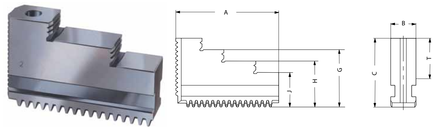
Tool group C 21 Type 574-27 One-piece reversible jaws, 3-jaw set, hardened, straight toothing - material: 16 MnCr 5
